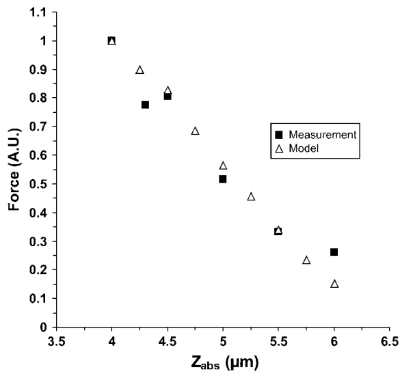
FIGURE 7 Fit of theoretical relationship to experimental results of force-distance. The only free parameter is the absolute initial distance Z where the AFM tip ended up at the end of the automatic approach. Black squares are a subset of measurements plotted in Fig. 5 (six leftmost points). The open triangles are the results of calculations from the model. The value of the parameter giving this fit is 2.5 \mu\text{m} , i.e., the depth to which the tip had originally penetrated into the field of cilia was 2.5 \mu\text{m} (see Fig. 5).
