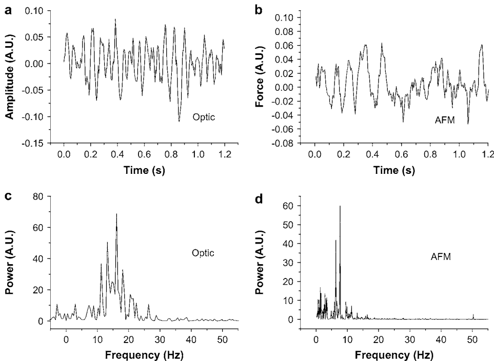
FIGURE 3 Optic and AFM measurement of cilia. ( a and c ) The optical signal, acquired on a sample beating with a relatively high-frequency ( \sim 15 Hz) raw signal and power spectrum, respectively. ( b and d ) AFM signal acquired from a different sample, beating at a lower-frequency ( \sim 8 Hz) raw signal and power spectrum, respectively. It is demonstrated that the FFT power spectrum faithfully reports the different frequencies (visually compare the raw signals in a and b ), both for the optical and AFM signals, despite the fact that the raw signal is less than periodical. The fluctuations in amplitude are typical of these cilia.
