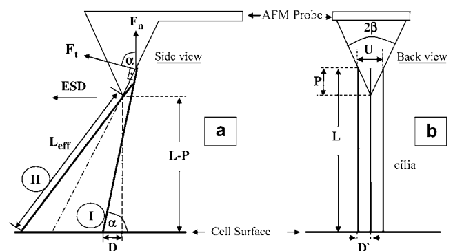
FIGURE 6 Schematic views of cilia and an AFM probe from two directions. (a) Side view, showing the AFM cantilever and tip aligned with the direction of the ESD. The dot-dashed oblique line is an imaginary continuation of the pyramid side to the cell's surface. Two cilia are also shown (wide lines), to the right and to the left of the dot-dashed line. (b) Three cilia beating in parallel with the ESD into the page and the cantilever of the AFM probe pointing out of the page (toward the reader). The symbols are explained in the text.
